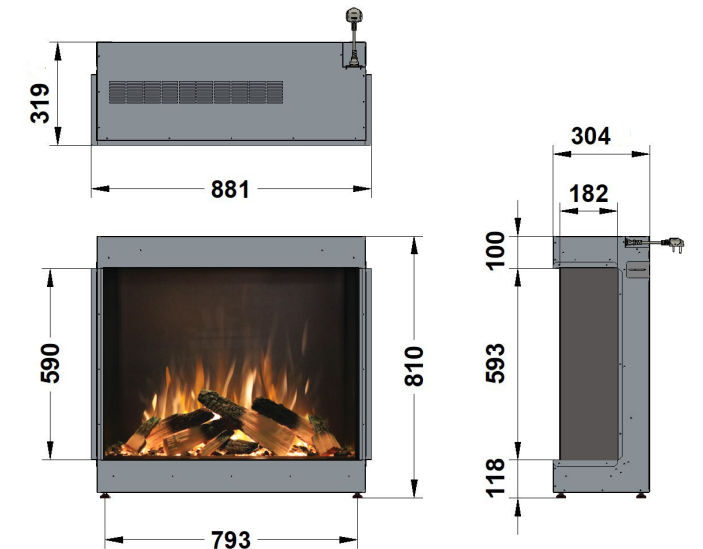
950 ASPECT - BAY
